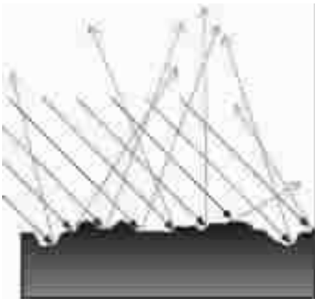
图5 四川巨棘龙鳞片横截面漫反射示意图 Fig. 5 Schematic map of diffuse reflections of the scale cross section of skin impressions of Gigantospinosaurus sichuanensis
