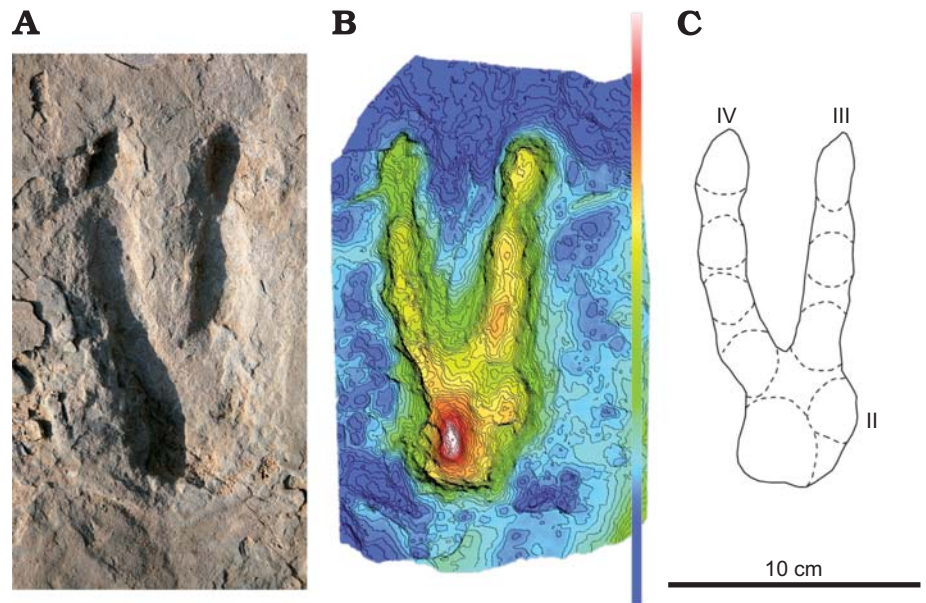
Fig. 2. Deinonychosaurian track Dromaeosauripus yongjingensis ichnosp. nov. holotype GSLTZP-S2-TE4L from the Early Cretaceous Yanguoxia track site, Gansu, China. A. Photograph. B. Computerized photogrammetry, with 0.2 mm contour lines; color banding reflects topography (blue-green, highest; red-white, lowest). Based on the photogrammetric maps from Xing et al. (2009: fig. 6). C. Outline drawing.
